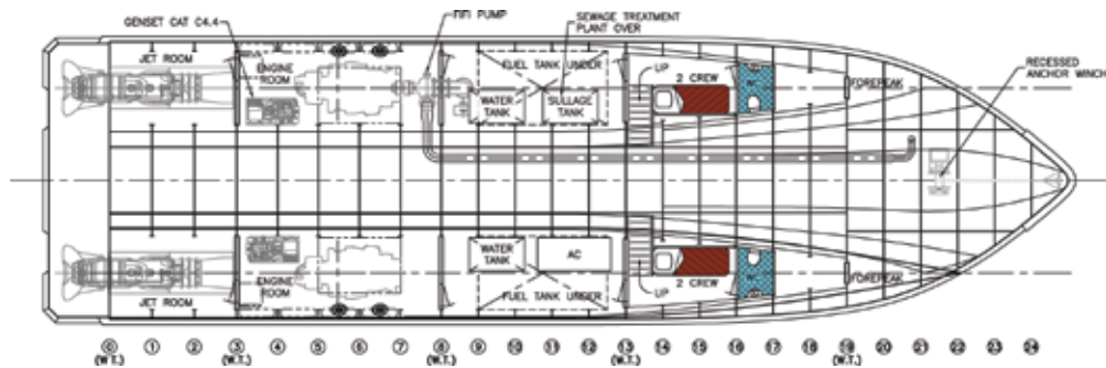
Hull plan
