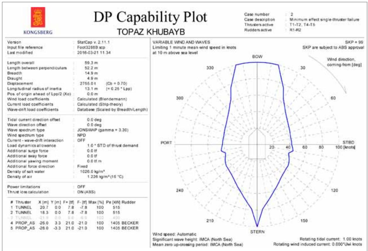
DP capability envelope for case 2
