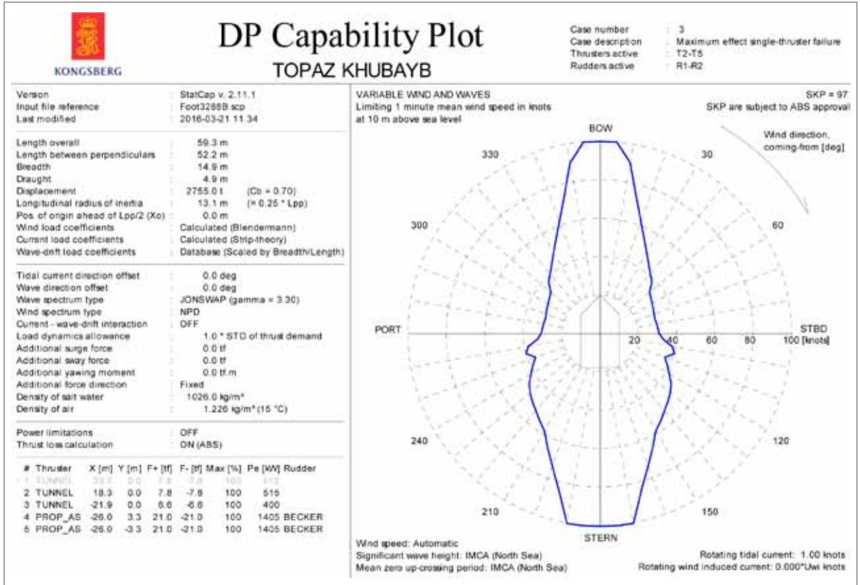
DP capability envelope for case 3
