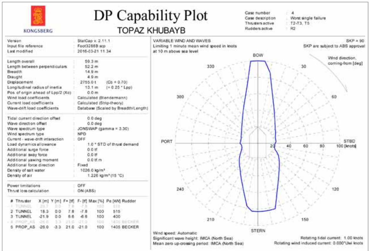
DP capability envelope for case 4
