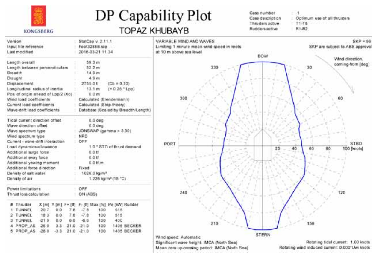
DP capability envelope for case 1
