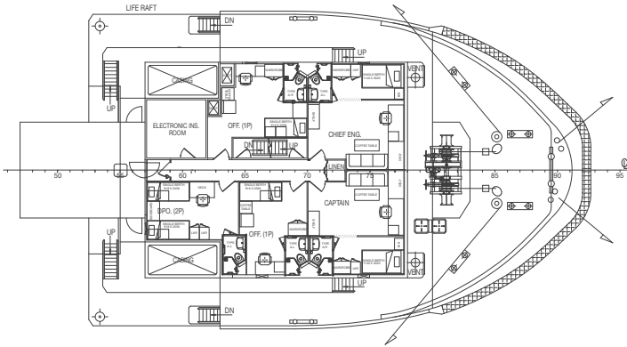
Forecastle deck
