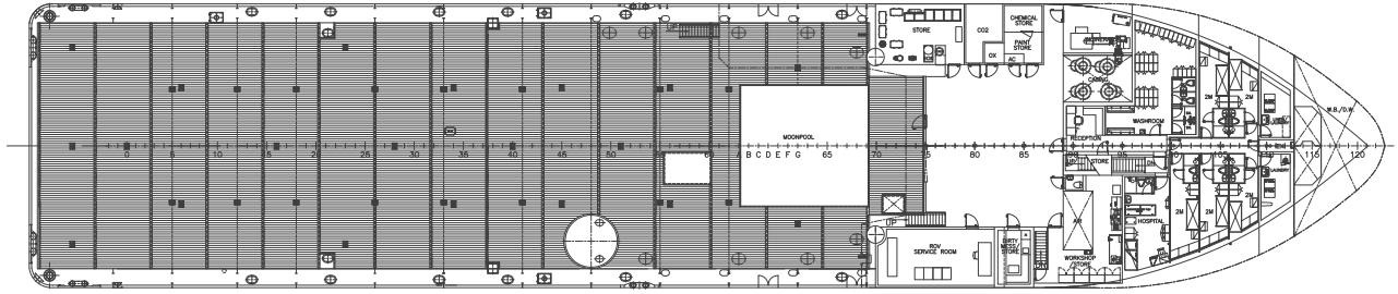
Main deck
