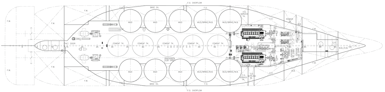
Tank top
