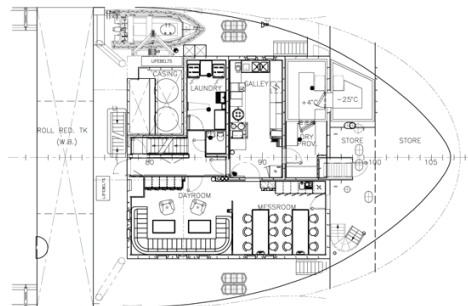
Forecastle deck
