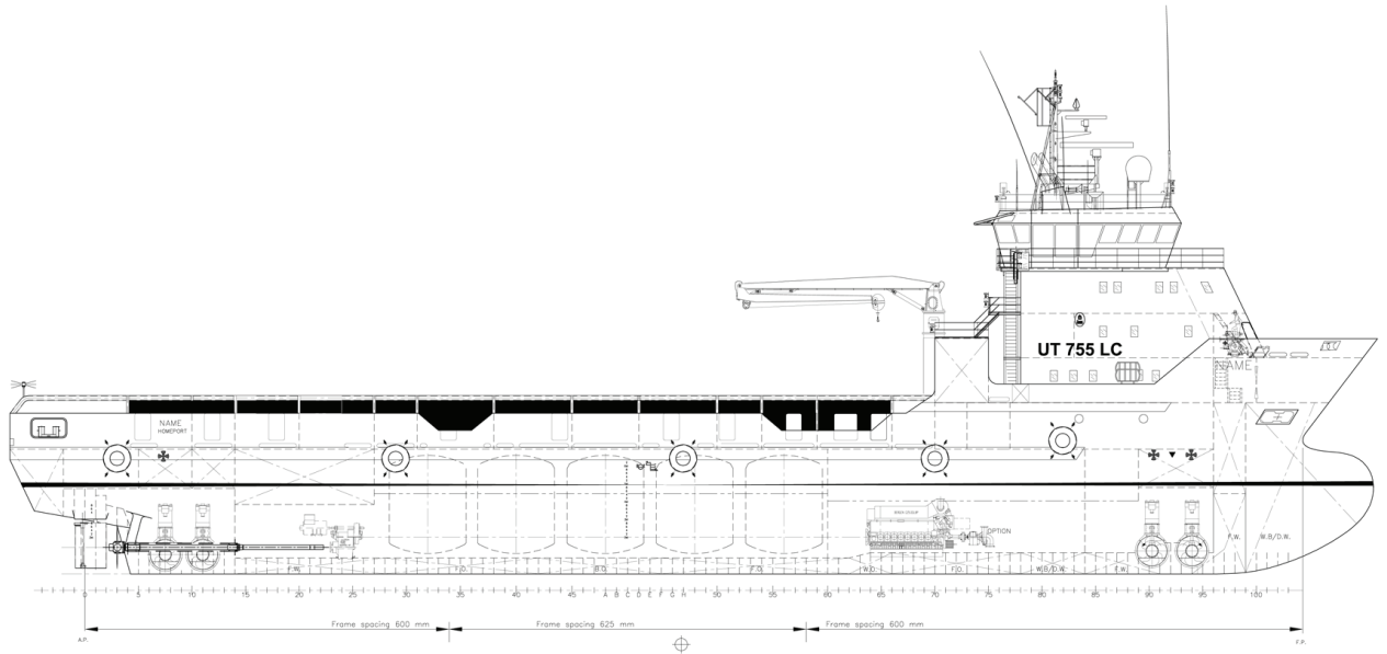
Outboard profile
