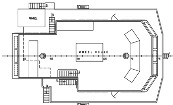
Nav. bridge deck
