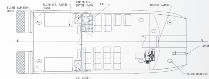
General arrangement for main deck
