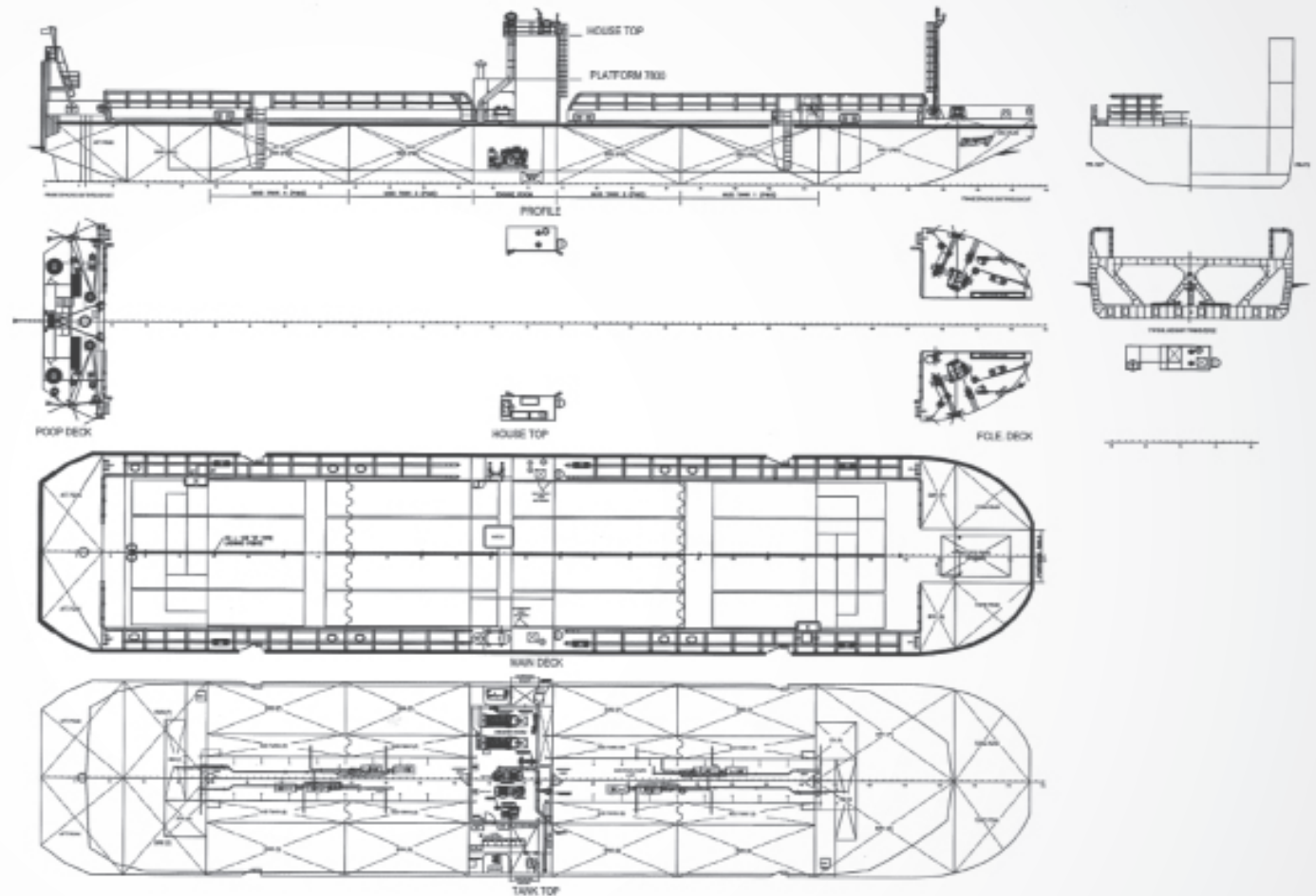
General arrangement
