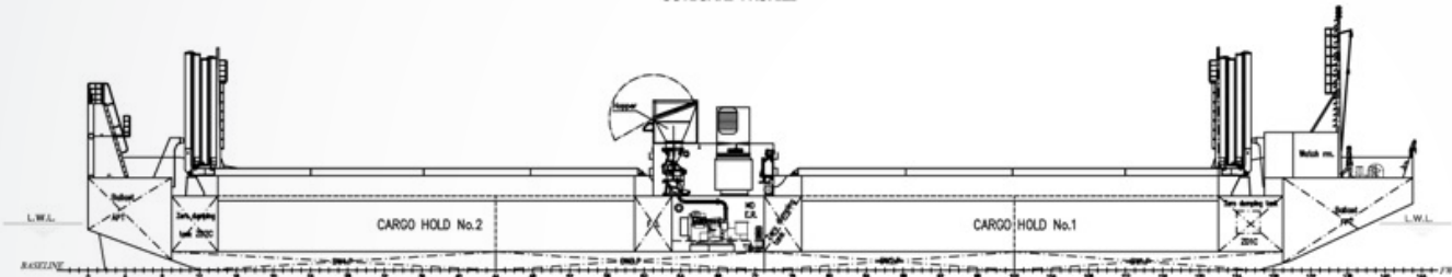
INBOARD PROFILE
