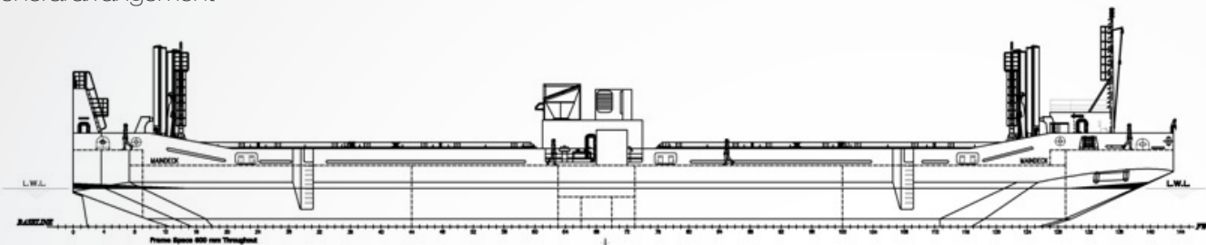
OUTBOARD PROFILE
