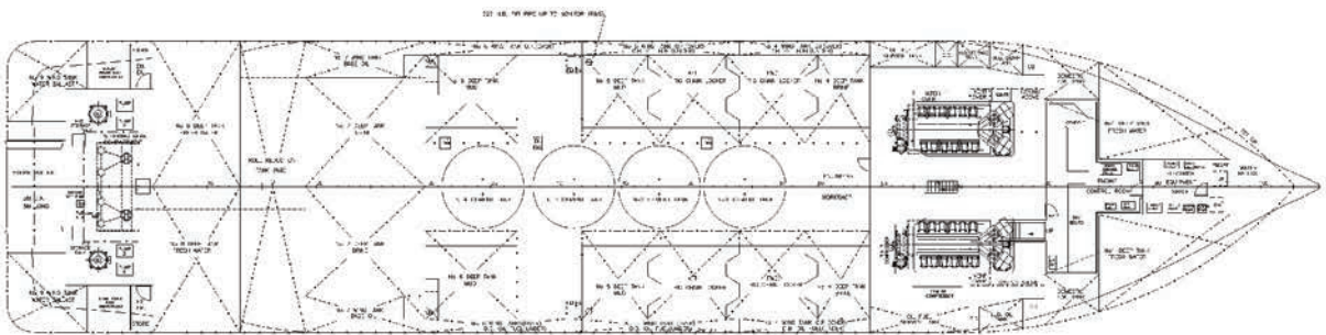
2 nd deck
