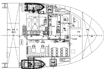
Forecastle deck
