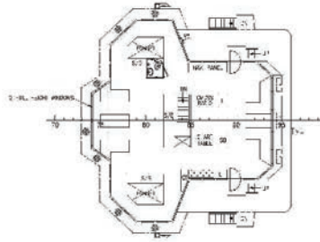
Wheelhouse deck
