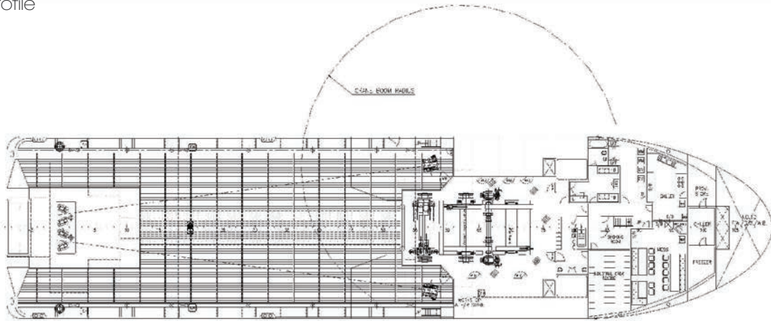
Main deck
