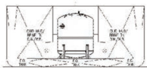
Section at cement tank
